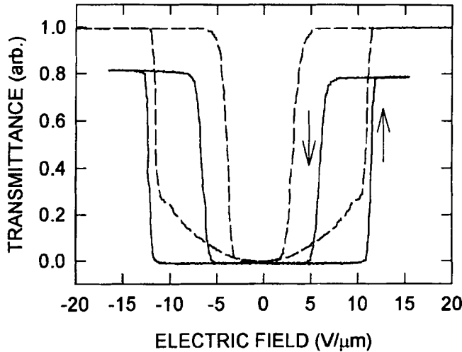
Figure 3: The double hysteresis in the EO transmittance measured with a triangular wave voltage at 0.5Hz. Solid and dashed lines represent AFLC and TAFLC, respectively.
