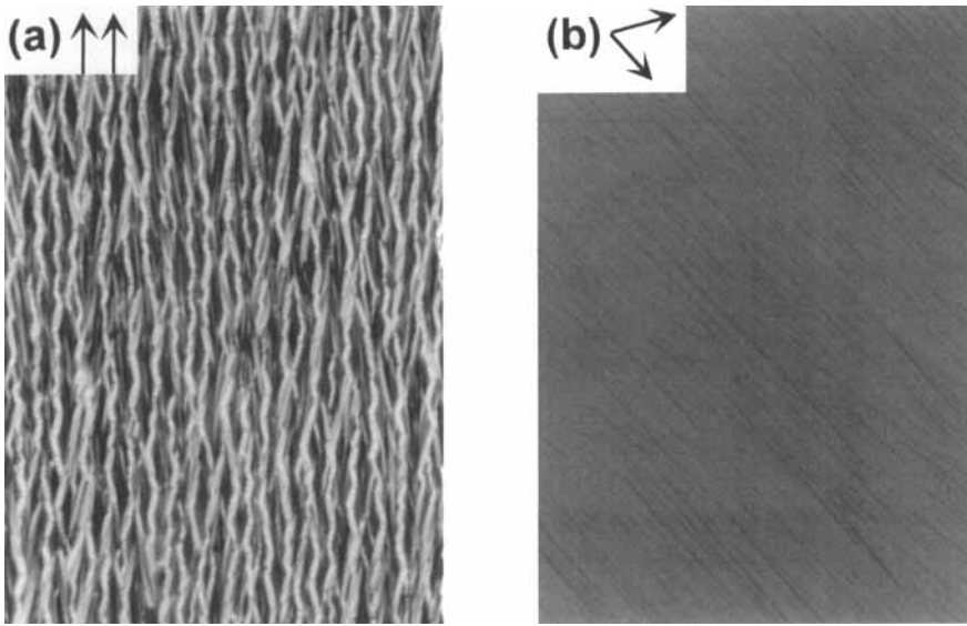
Figure 1: Typical textures of (a) the planar and (b) the 54^\circ twisted AFLC cells, observed under crossed polarizers. (See Color Plate I).
